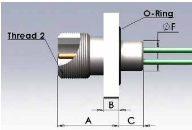
CCR (5502)
