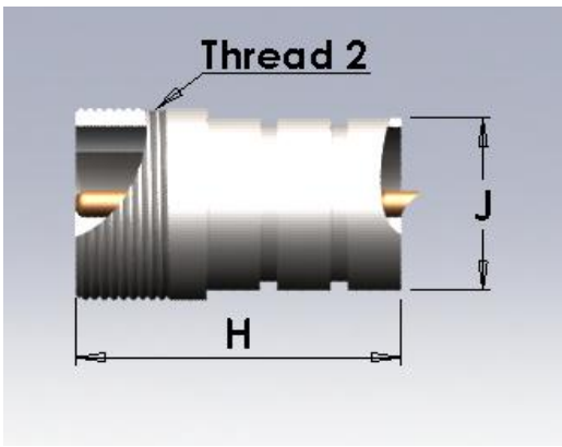
CCR-AT (55A2)
