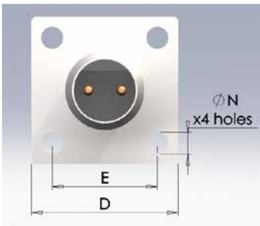
CCR-AT (55A2)
