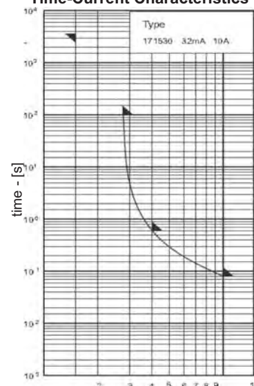
Time-Current Characteristics
