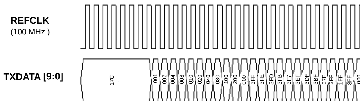
Figure 7-9. Generated Clock and Data Signals for Encoder Bypass Mode from DG2020
