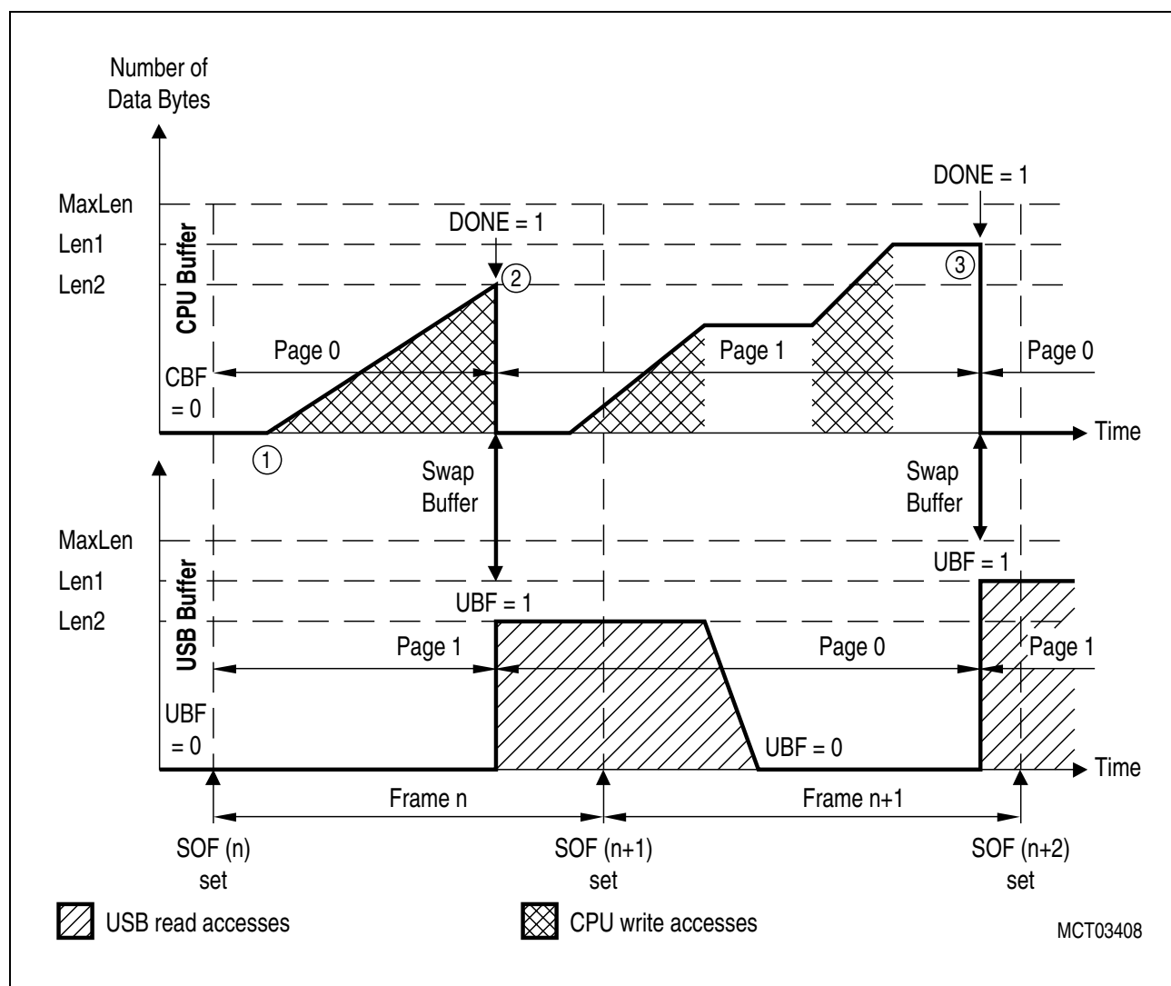
Figure 22-15 Dual Buffer Mode USB Read Access : Buffer Switching by Setting Bit DONE
