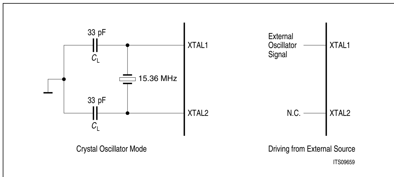
Figure 26-1 Oscillator Circuit
