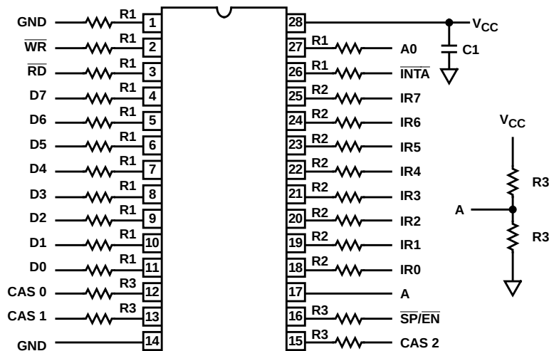
MR82C59A CLCC
