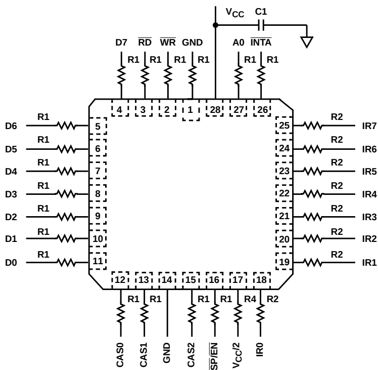
MR82C59A CLCC
