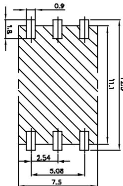
10027621-003 RECOMMENDED PCB LAYOUT; SCALE: 5/1
