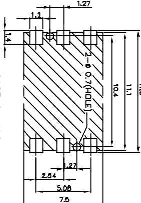
10027621-002 RECOMMENDED PCB LAYOUT; SCALE: 5/1
