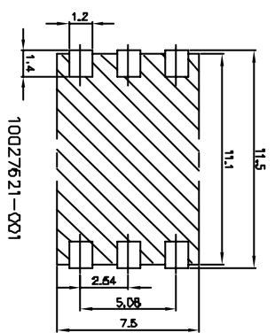
10027621-001 RECOMMENDED PCB LAYOUT; SCALE: 5/1
