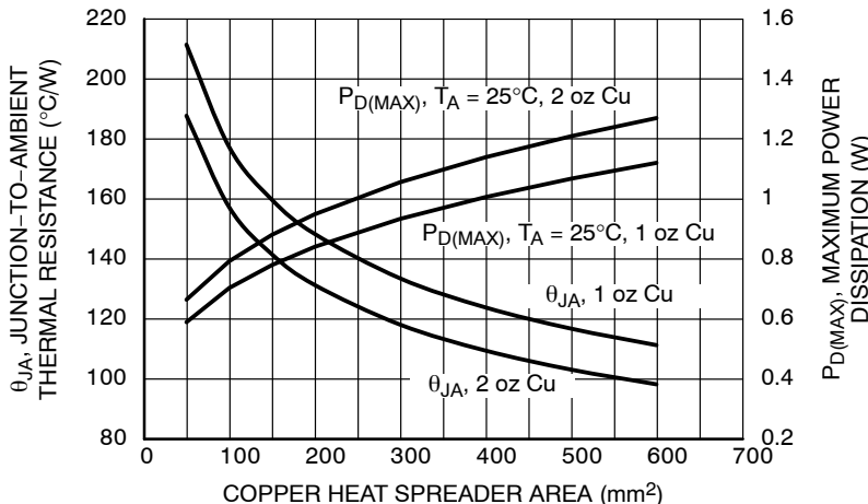
Figure 66. \theta_{JA} and P_{D(MAX)} vs. Copper Area (WDFN6)
