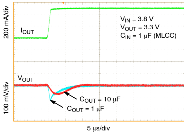
Figure 56. Load Transient Response – Rising Edge, V_{OUT} = 3.3 V, I_{OUT} = 1 mA to 500 mA, C_{OUT} = 1 μF, 10 μF
