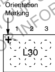
CM1230-04 6-bump CSP Package
