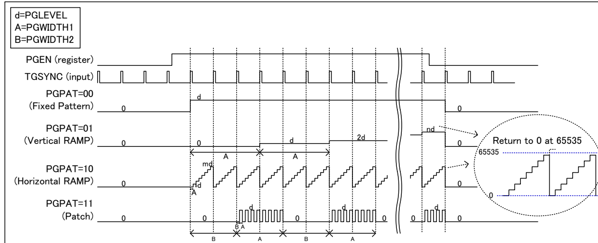
Figure 32 Test Pattern Output Data Formats
