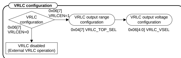
Figure 40 VRCL Configuration
