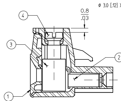
SECT. Z-Z
