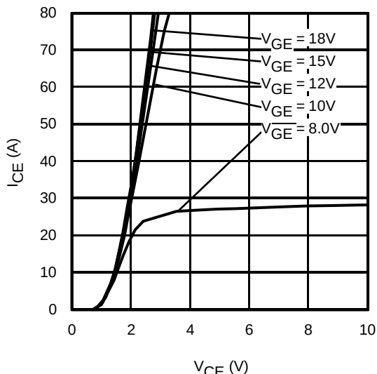
Fig. 5 - Typ. IGBT Output Characteristics T_J = -40^\circ\text{C} ; t_p = 30\mu s
