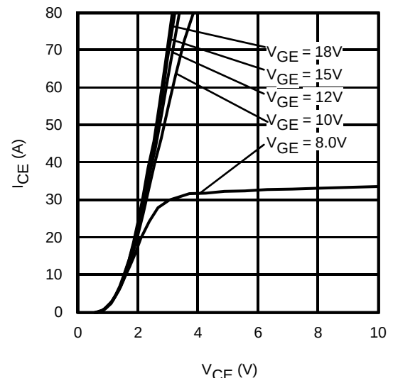
Fig. 6 - Typ. IGBT Output Characteristics T_J = 25^\circ\text{C} ; t_p = 30\mu s
