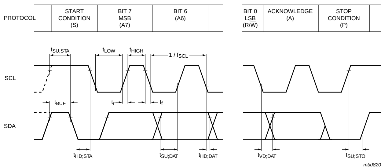
Fig 21. I 2 C bus timing diagram; rise and fall times refer to V_{IL} and V_{IH}
