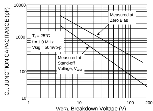
FIG. 6 - TYPICAL JUNCTION CAPACITANCE UNI-DIRECTIONAL
