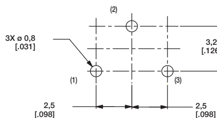
PCB LAYOUT RECOMMENDED
