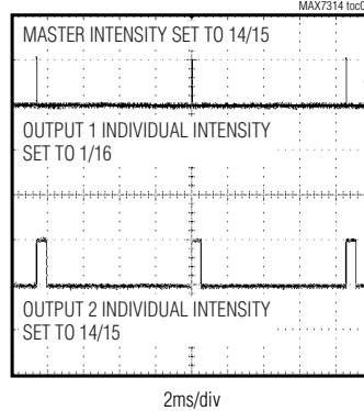
SCOPE SHOT OF 2 OUTPUT PORTS
