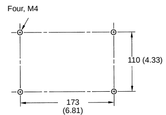
Mounting Holes
