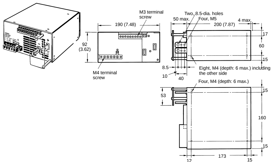
Mounting Holes Side View
