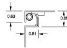
Cross Section of 16 Gauge Body and Door
