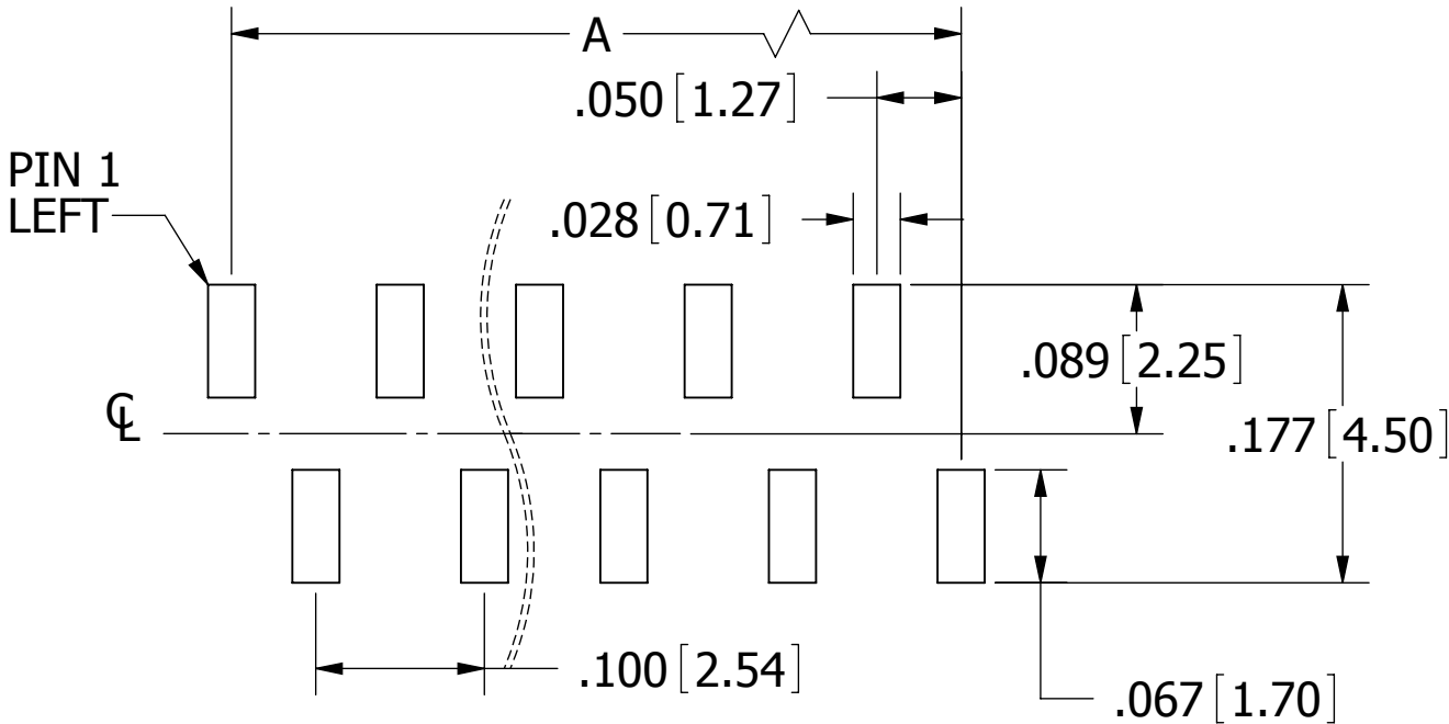
RECOMMENDED PCB SMD LAYOUT GRP B _ 1 VW T C-RC
