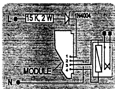
Single Resistor PSU
