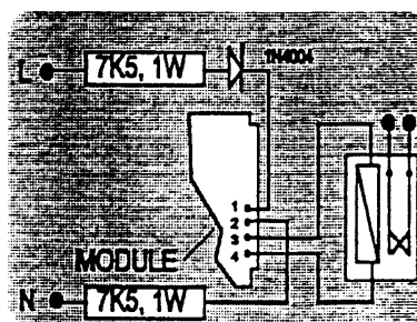
Two Resistor PSU - gives Optimum EMC Performance
