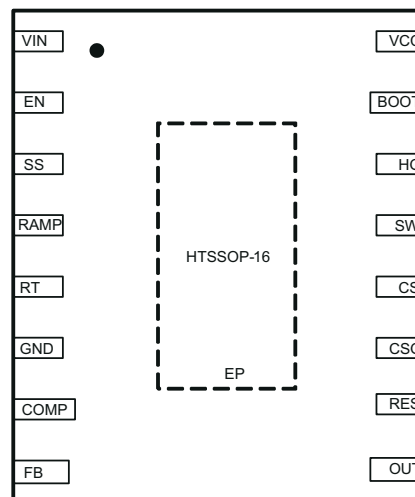
Figure 5-2. 16-Pin PWP Package (Restart Version) (Top View)
