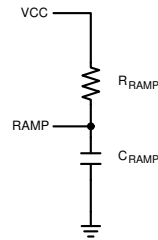
Figure 8-3. Additional Slope Compensation for V_{OUT} > 5\text{ V}
