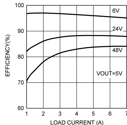
Typical Application Circuit Efficiency
