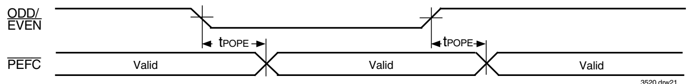
Figure 21. ODD/ \overline{EVEN} to \overline{PEFC} Timing
