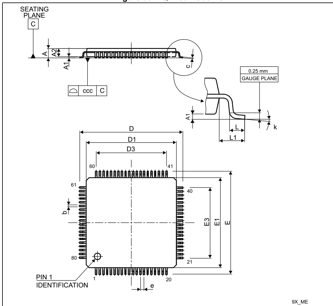
Figure 66. LQFP80 - Outline
