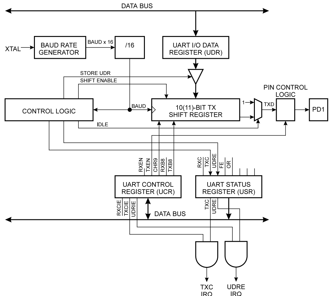
Figure 19. UART Transmitter
