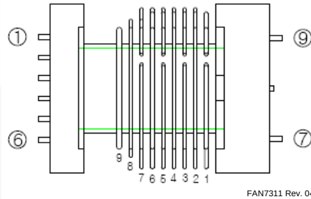
Figure 11. Transformer Schematic
