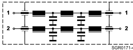
Circuit diagram 1
