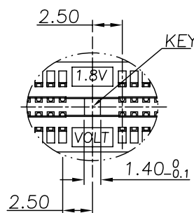
DETAIL A (1.8V) SCALE 2:1
