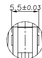
DETAIL D SCALE 2:1
