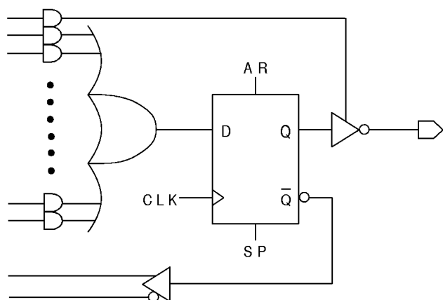
ACTIVE LOW
