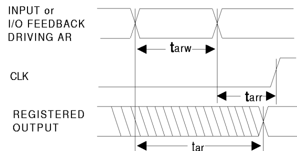
Asynchronous Reset
