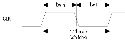
Clock Width
