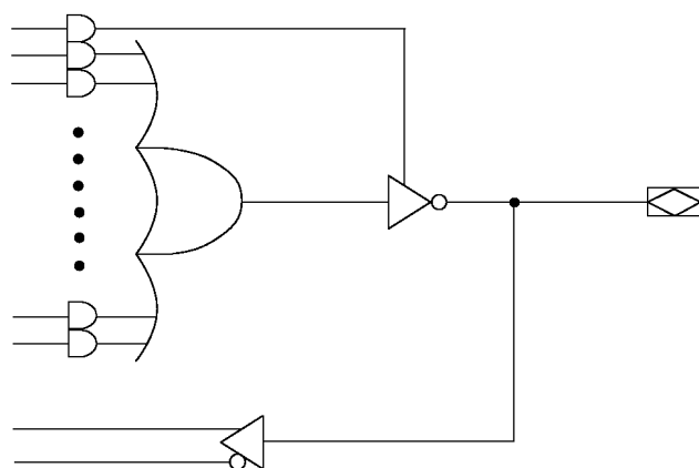
ACTIVE LOW
