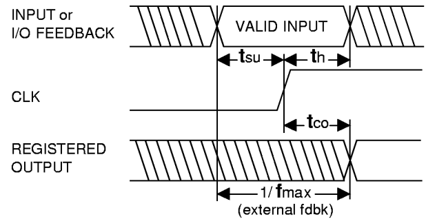
Registered Output
