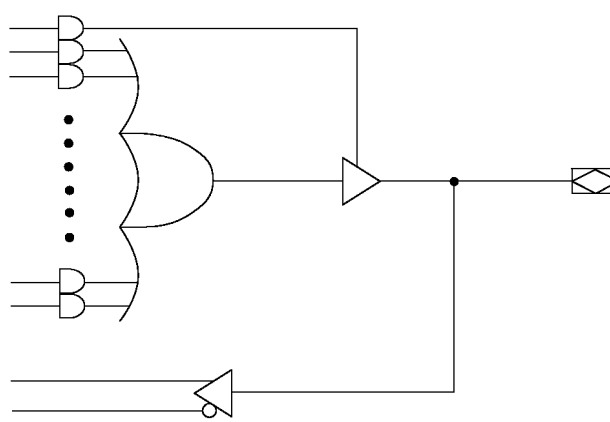
ACTIVE HIGH
