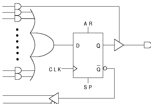
ACTIVE HIGH
