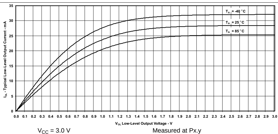
Figure 3. Typical Low-Level Output Current vs Low-Level Output Voltage
