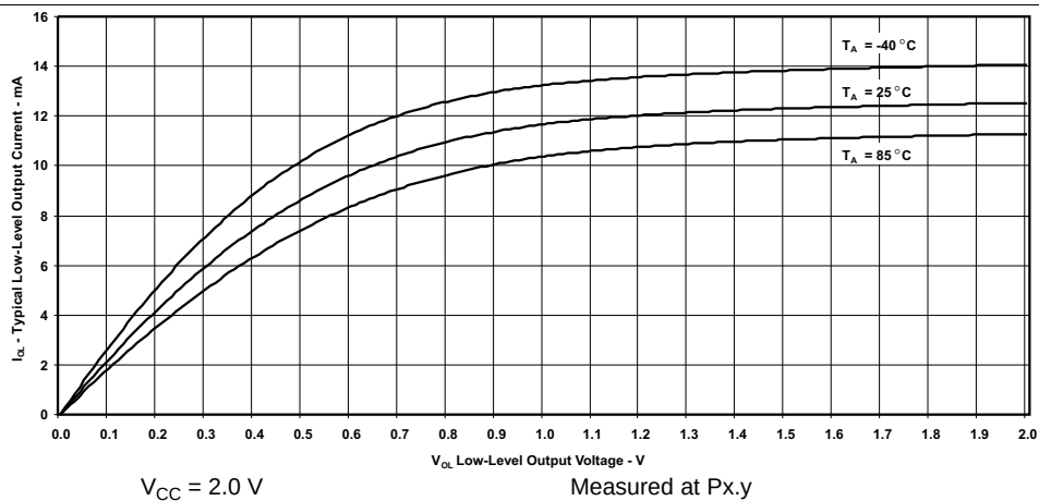
Figure 2. Typical Low-Level Output Current vs Low-Level Output Voltage
