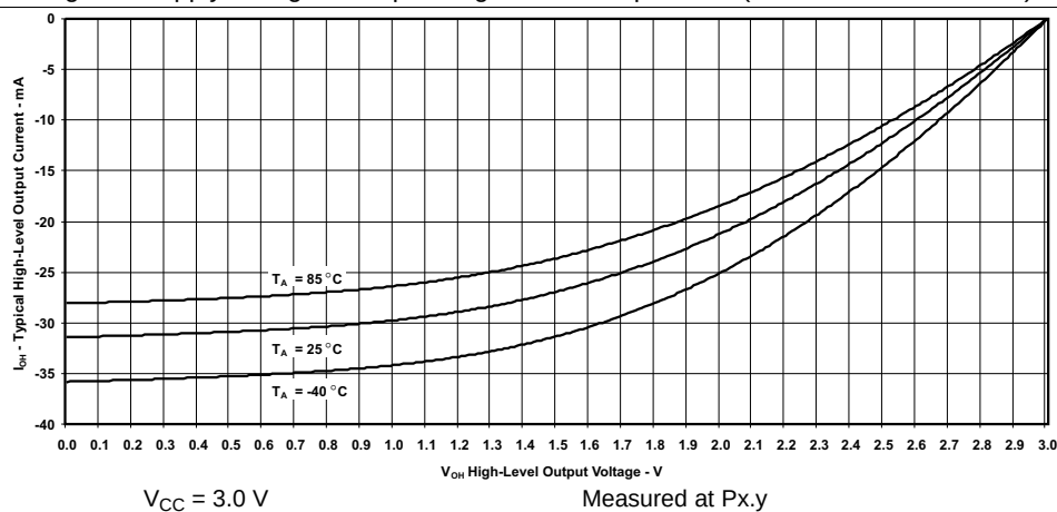
Figure 5. Typical High-Level Output Current vs High-Level Output Voltage
