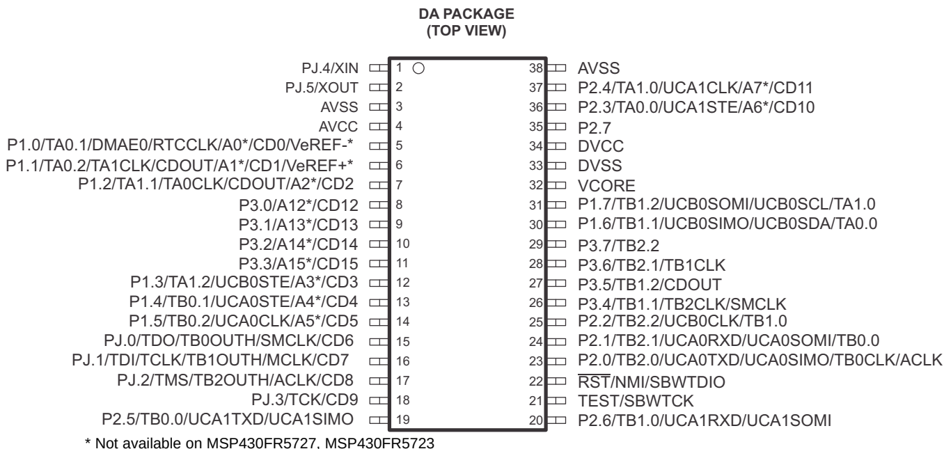
Figure 4-2. 38-Pin DA Package
