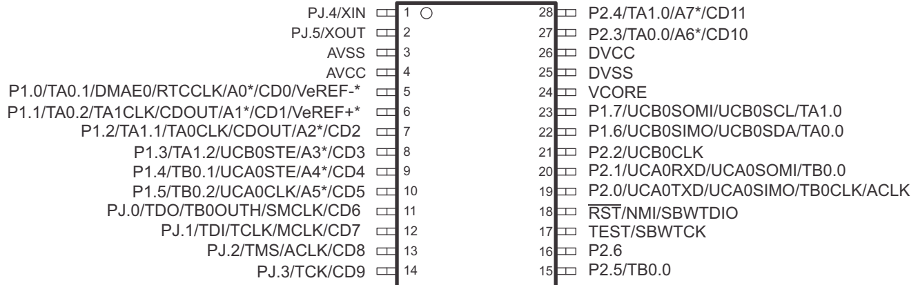
Figure 4-4. 28-Pin PW Package
