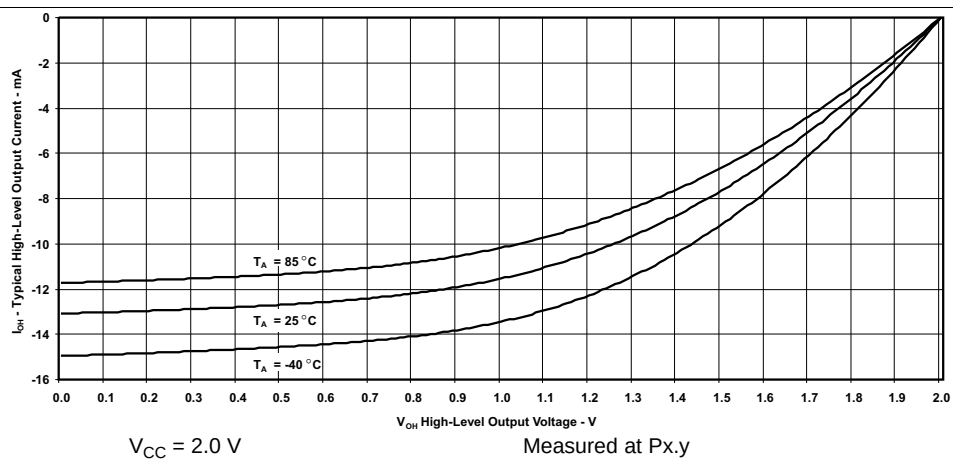
Figure 4. Typical High-Level Output Current vs High-Level Output Voltage
