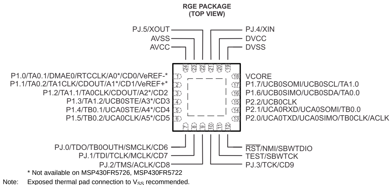
Figure 4-3. 24-Pin RGE Package
