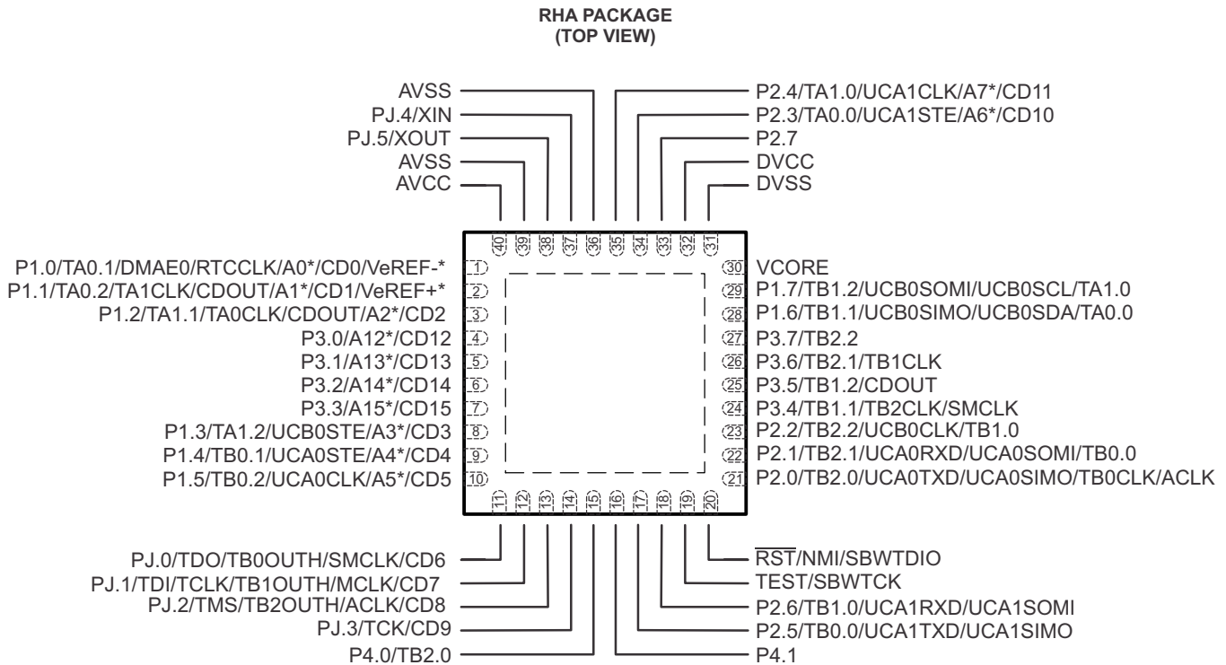
Figure 4-1. 40-Pin RHA Package
