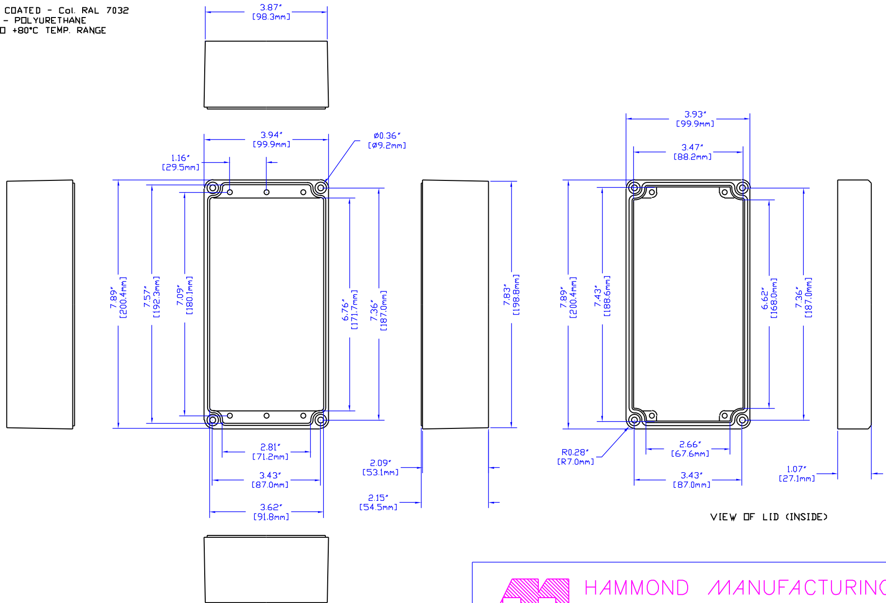
VIEW OF BOX (LID REMOVED)
