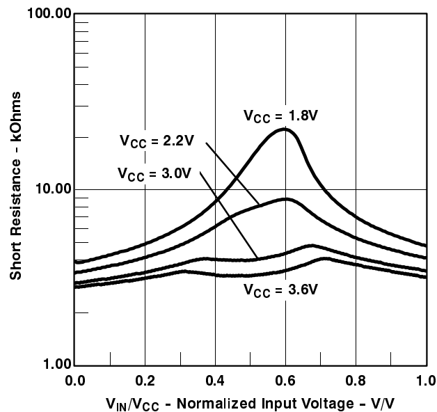
Figure 30. Short Resistance vs V_{IN}/V_{CC}
