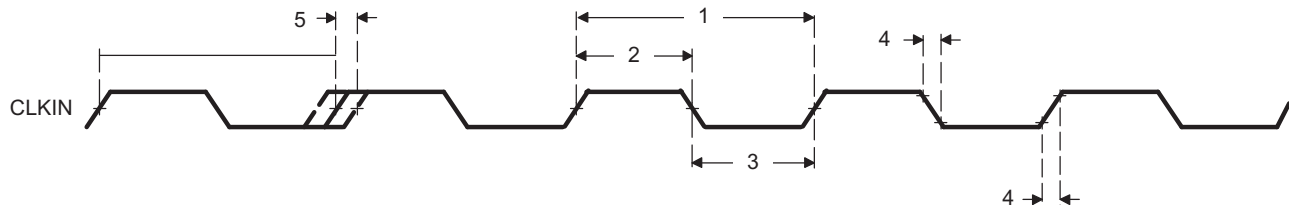
Figure 6-6. CLKIN1 Timing
