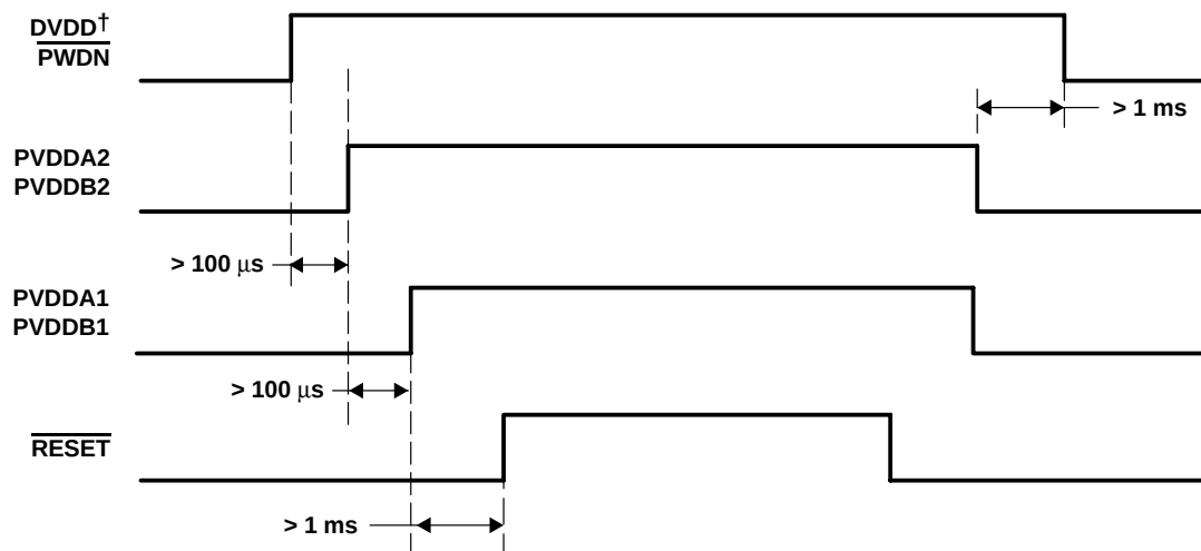
Figure 3. Power-Up/Power-Down Sequence
