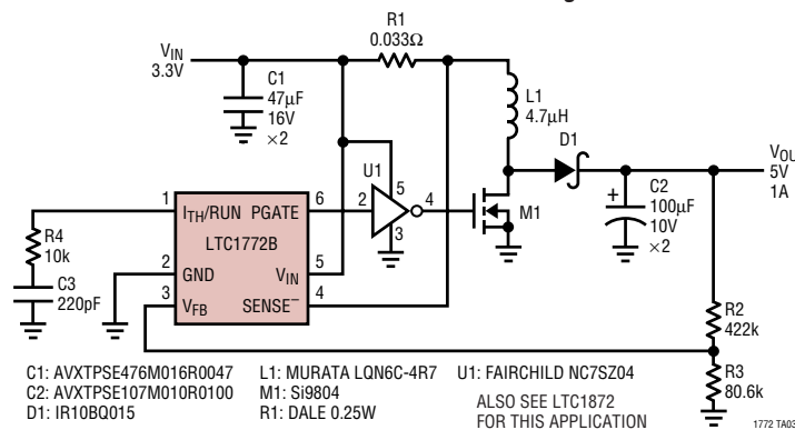
LTC1772B 3.3V to 5V/1A Boost Regulator
