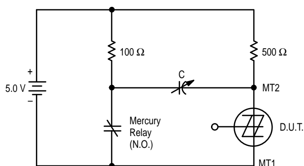
FIGURE 9 – TURN-OFF TIME TEST CIRCUIT
