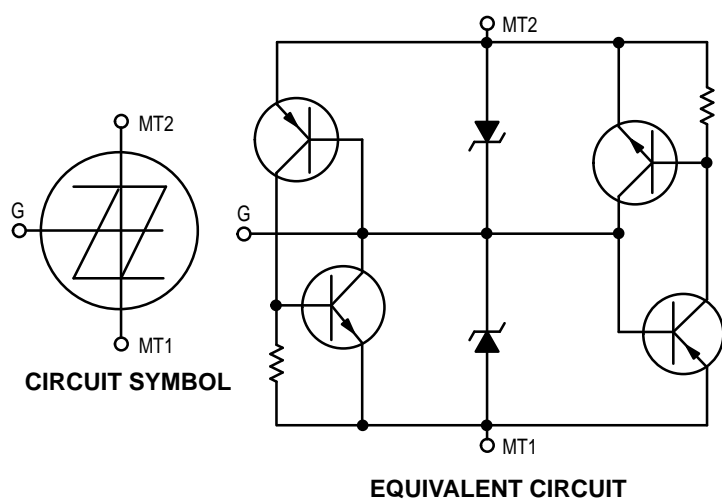
FIGURE 10 – DEVICE EQUIVALENT CIRCUIT, CHARACTERISTICS AND SYMBOLS
