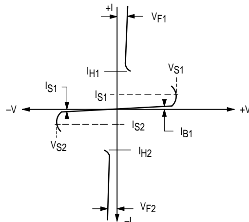
FIGURE 10 – DEVICE EQUIVALENT CIRCUIT, CHARACTERISTICS AND SYMBOLS
