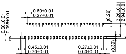
Recommended metal mask pattern Metal mask thickness: When 120μm (Front terminal portion opening area ratio: 50%) (Back terminal portion opening area ratio: 51%) (Soldering terminal portion opening area ratio: 100%)
