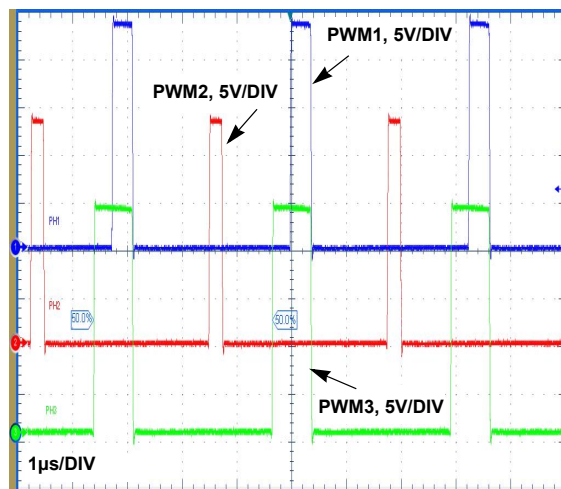
FIGURE 15. PHASE NODE PWM WAVEFORMS, V_{IN} = 24V
