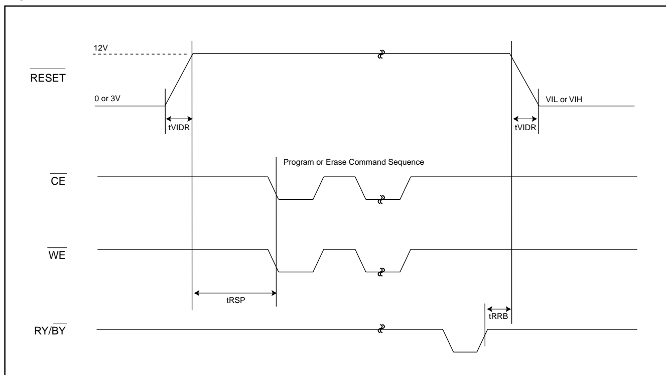
Fig 18. TEMPORARY SECTOR GROUP UNPROTECT WAVEFORMS
