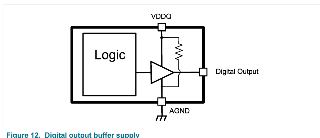
Figure 12. Digital output buffer supply
