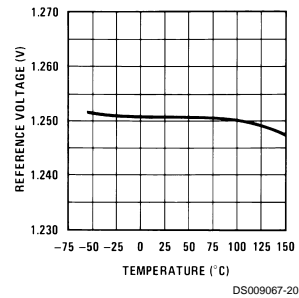
Temperature Stability
