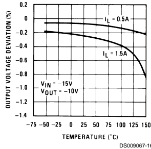
Load Regulation
