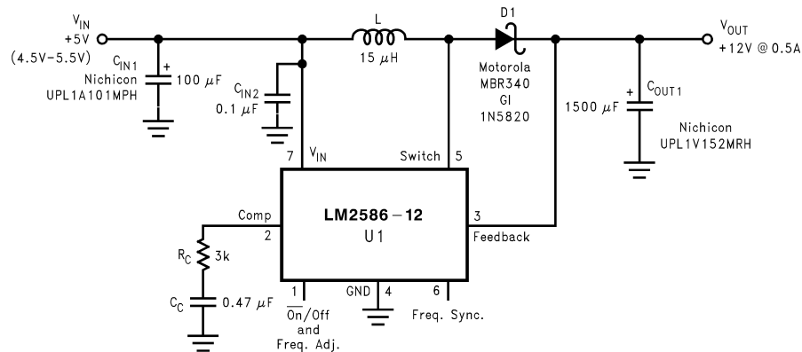
Figure 34. +5V to +12V Boost Regulator
