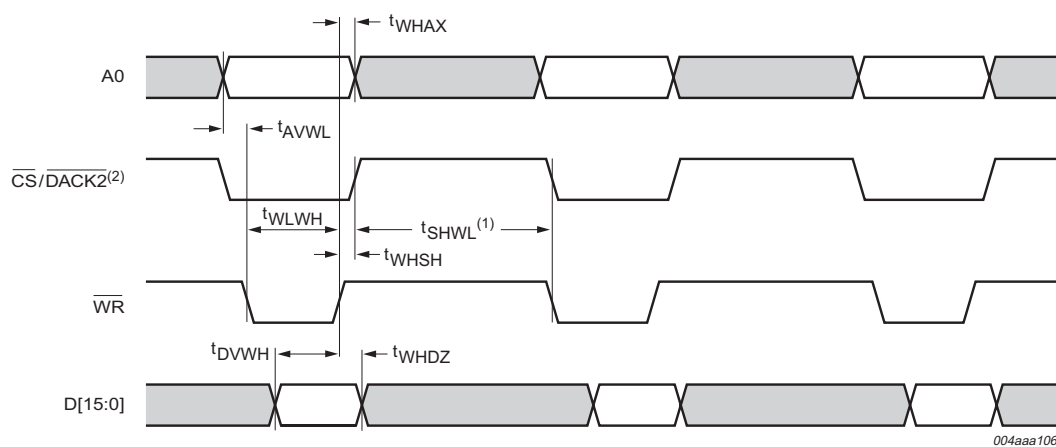
Fig 51. DC Programmed interface write timing (I/O and 8237 compatible DMA).
