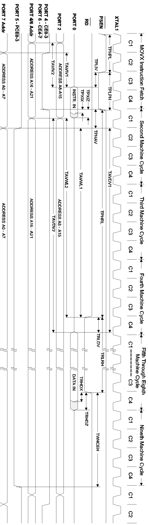
Non-Multiplexed Address/Data 9 Cycle PCEN-3 MOVX Read
