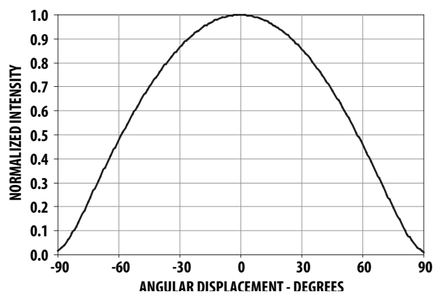
Figure 11. Radiation Pattern
