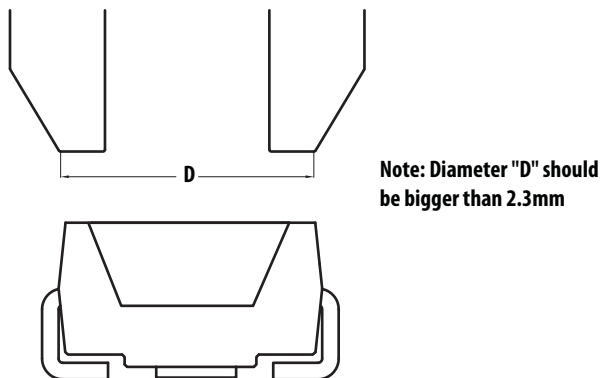
Figure 12. Recommended Pick and Place Nozzle Size
