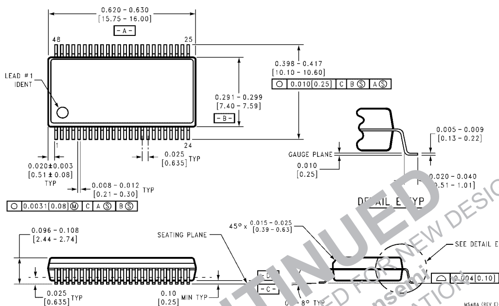
48-Lead Small Shrink Outline Package (SSOP), JEDEC MO-118, 0.300" Wide Package Number MS18A
