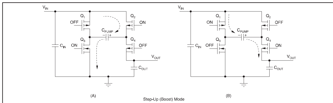
Figure 1. Simplified Schematic of the SN0304078 Operating in the Step-Up or Boost Mode
