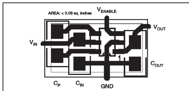
Figure 3. Suggested PCB Design for Minimum Ripple
