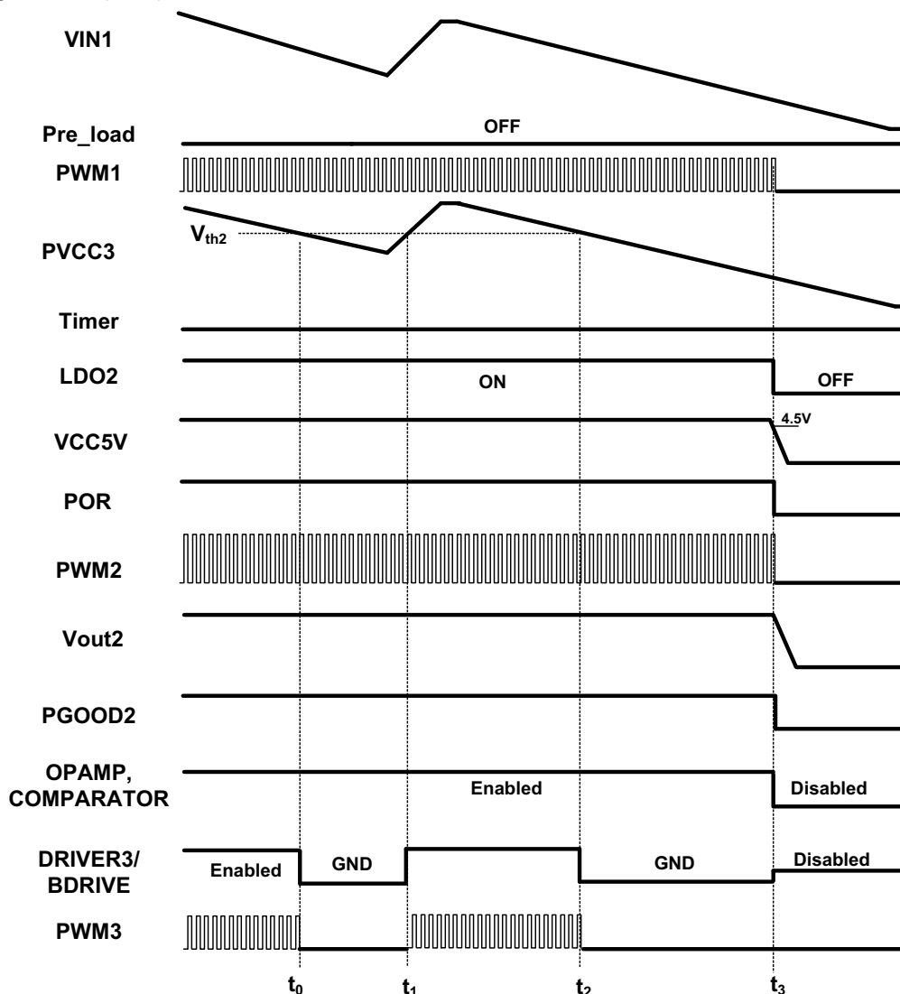
FIGURE 27. POWER-DOWN SEQUENCE
