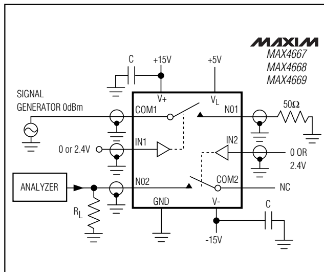
Figure 5. Crosstalk Test Circuit
