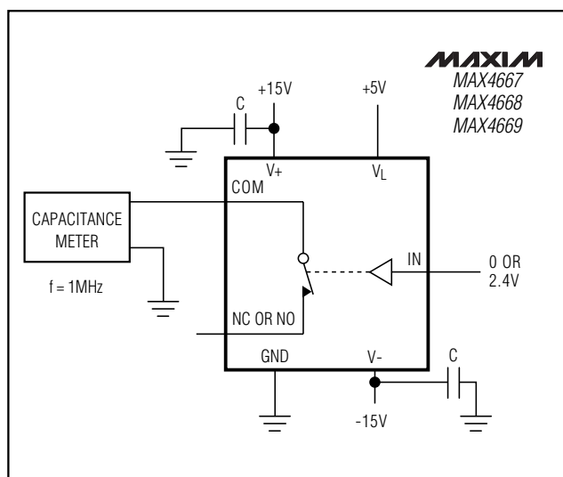
Figure 7. Switch On-Capacitance Test Circuit
