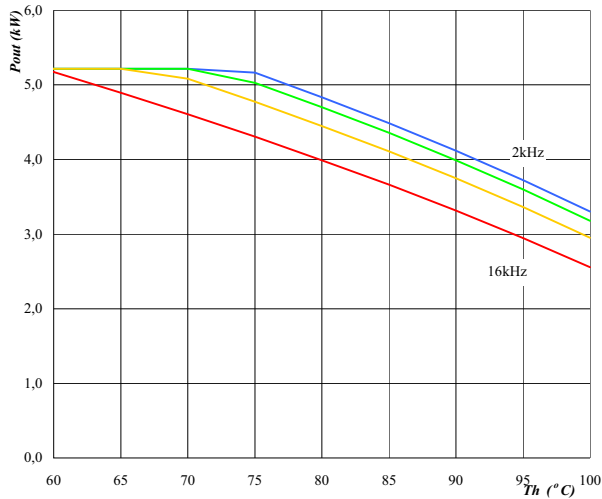
Figure 9. Typical available electric peak output power as a function of heatsink temperature
