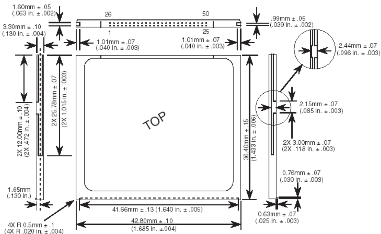
FIGURE 8-1: Physical dimension
