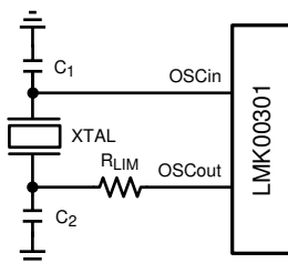
Figure 9-5. Crystal Interface
